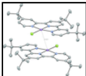
Fig. 2. Mercury (Macrae et al. , 2008) rendition of head-to-tail packing with Pt—Pt' distance 3.5214 (2) Å. Symmetry operation for the primed atom: 1-x, 1-y, 1-z
